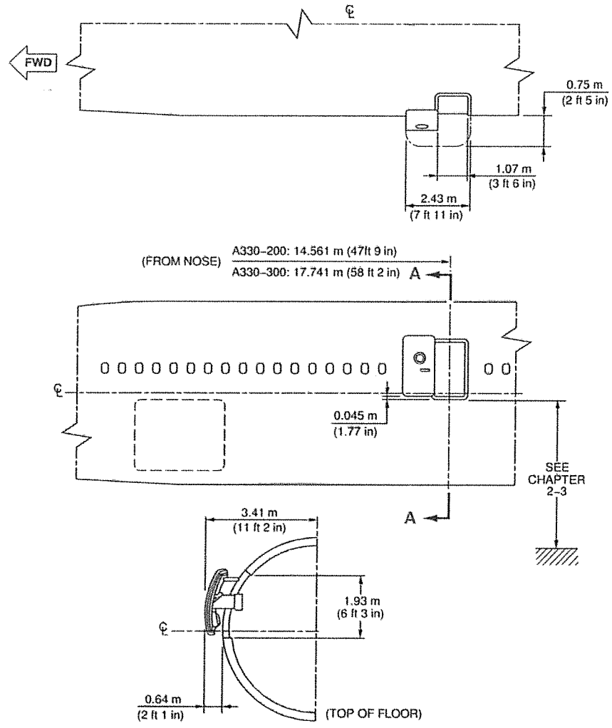
Mid Passenger / Crew Door FIGURE-2-7-2-991-001-A01
