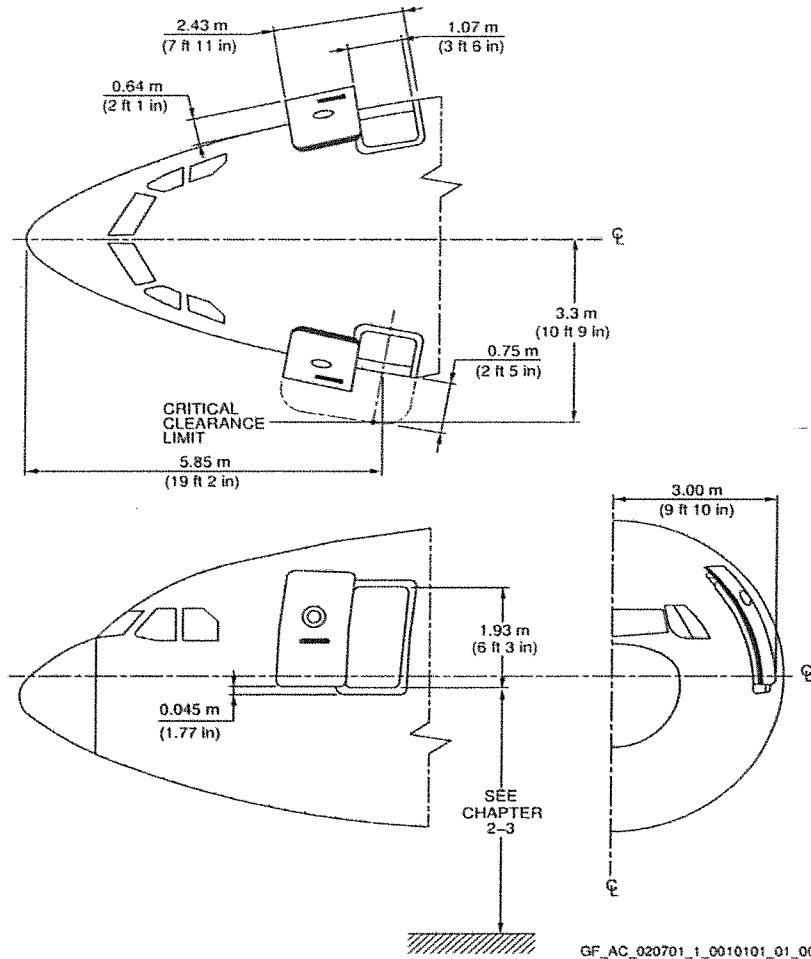
Forward Passenger / Crew Doors FIGURE-2-7-1-991-001-A01
