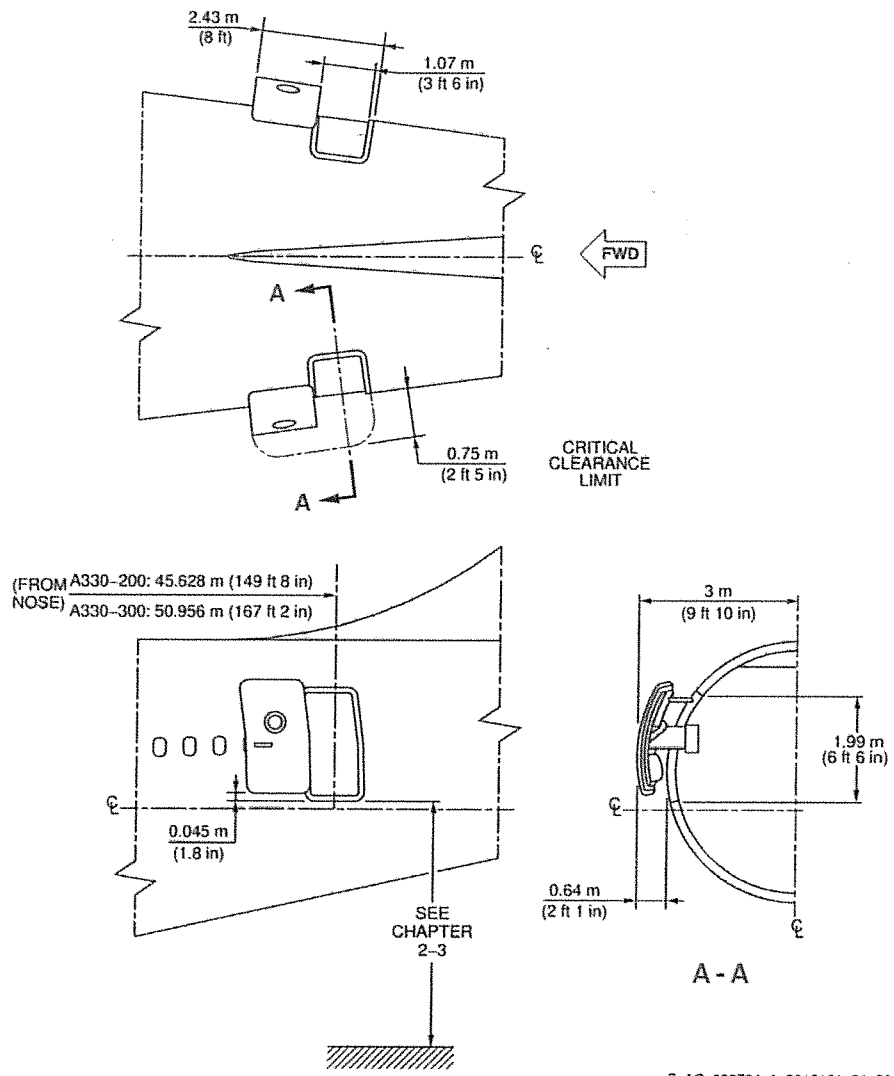
Aft Passenger / Crew Doors FIGURE-2-7-4-991-001-A01
