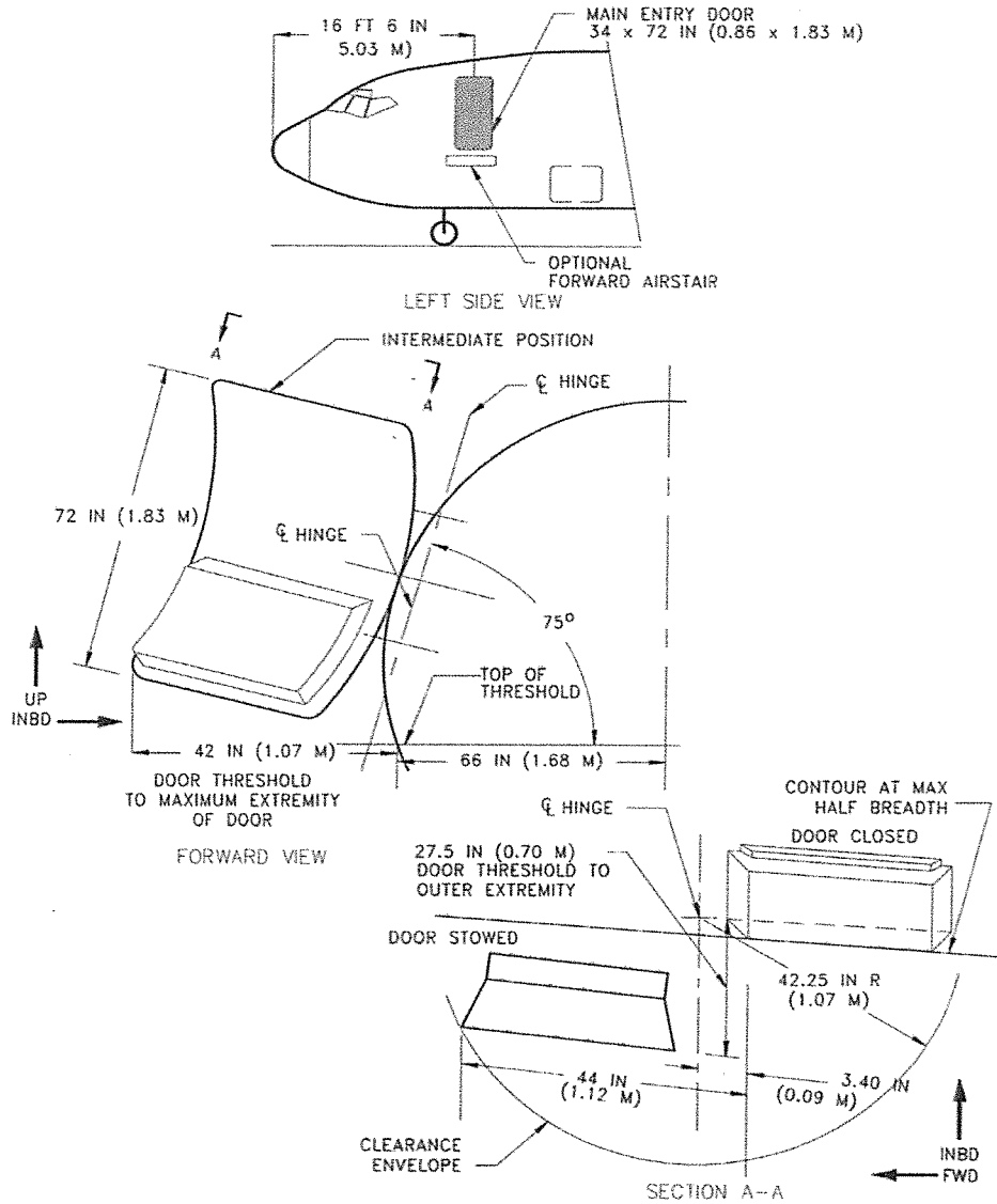
2.7.1 DOOR CLEARANCES - FORWARD MAIN ENTRY DOOR NO. 1 MODEL 737, ALL MODELS
