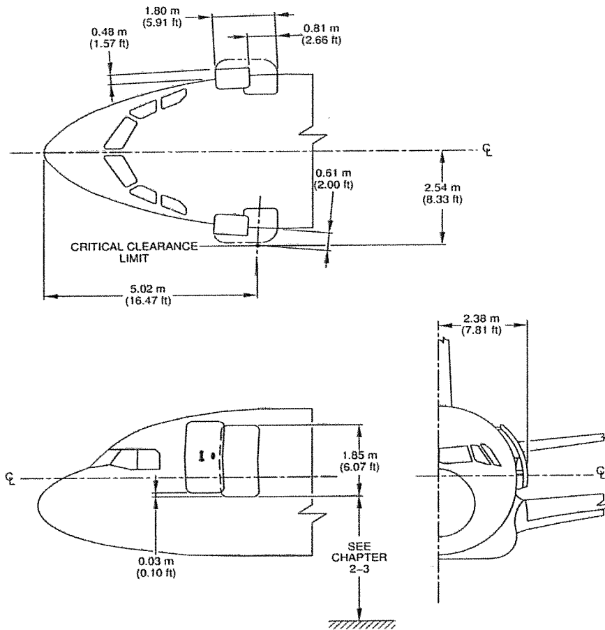
Doors Clearances Forward Passenger/Crew Doors FIGURE-2-7-0-991-022-A01
